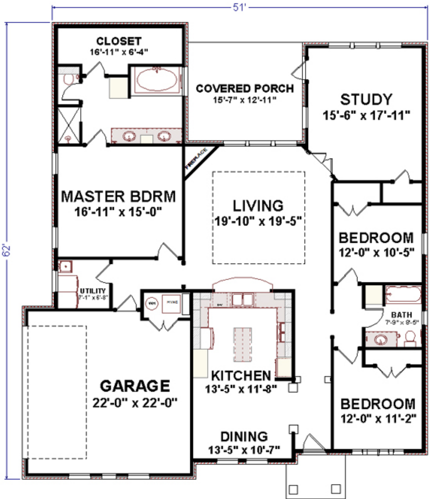
2327 FLOOR PLAN
