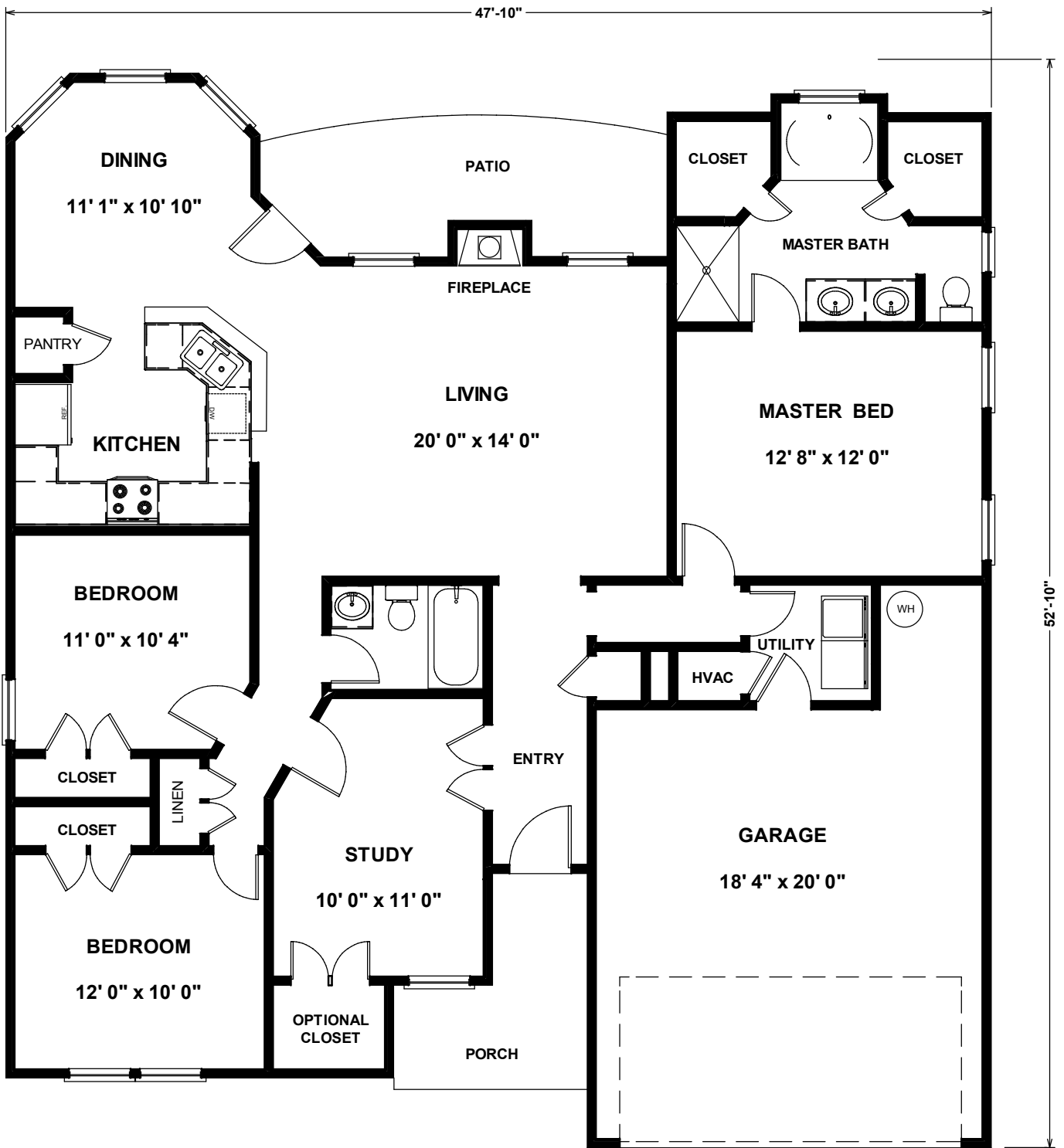
1675 FLOOR PLAN
